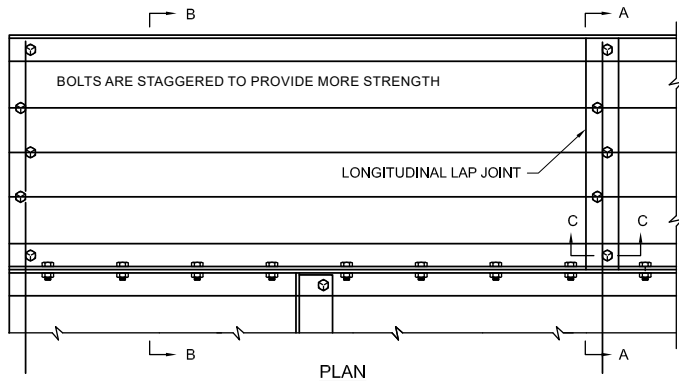
2-Flange Lap Joint
